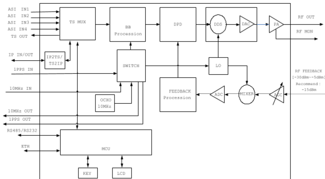
Figure 1. Exciter Diagram
