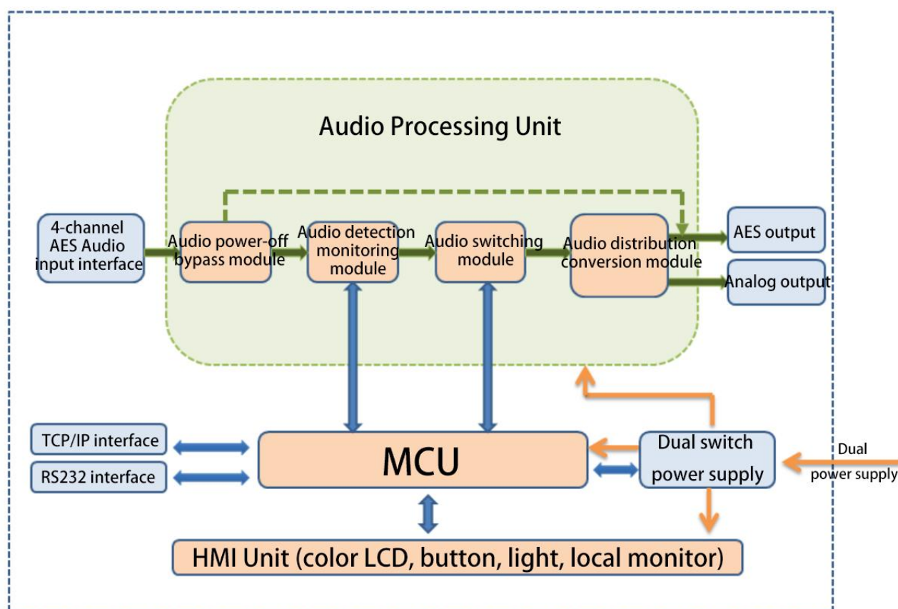
ZHC348-0411SZ Intelligent Audio Switcher Diagram
